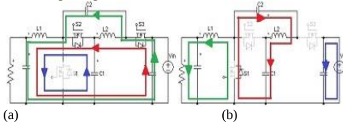
Fig. 4. Step-down mode (a) Mode-1 (b) Mode-2
