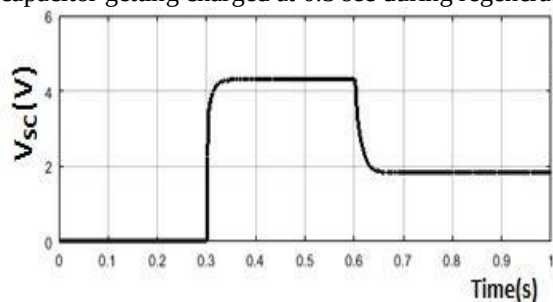
Fig. 10. Super-capacitor voltage
